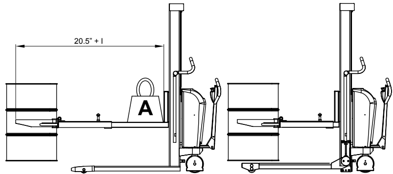
Very flexible handling situation - drums can be gripped from various run-in angles.
