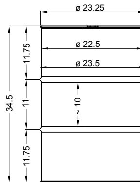
Standard steel drum (DS/EN 209 and DS/EN 210).
